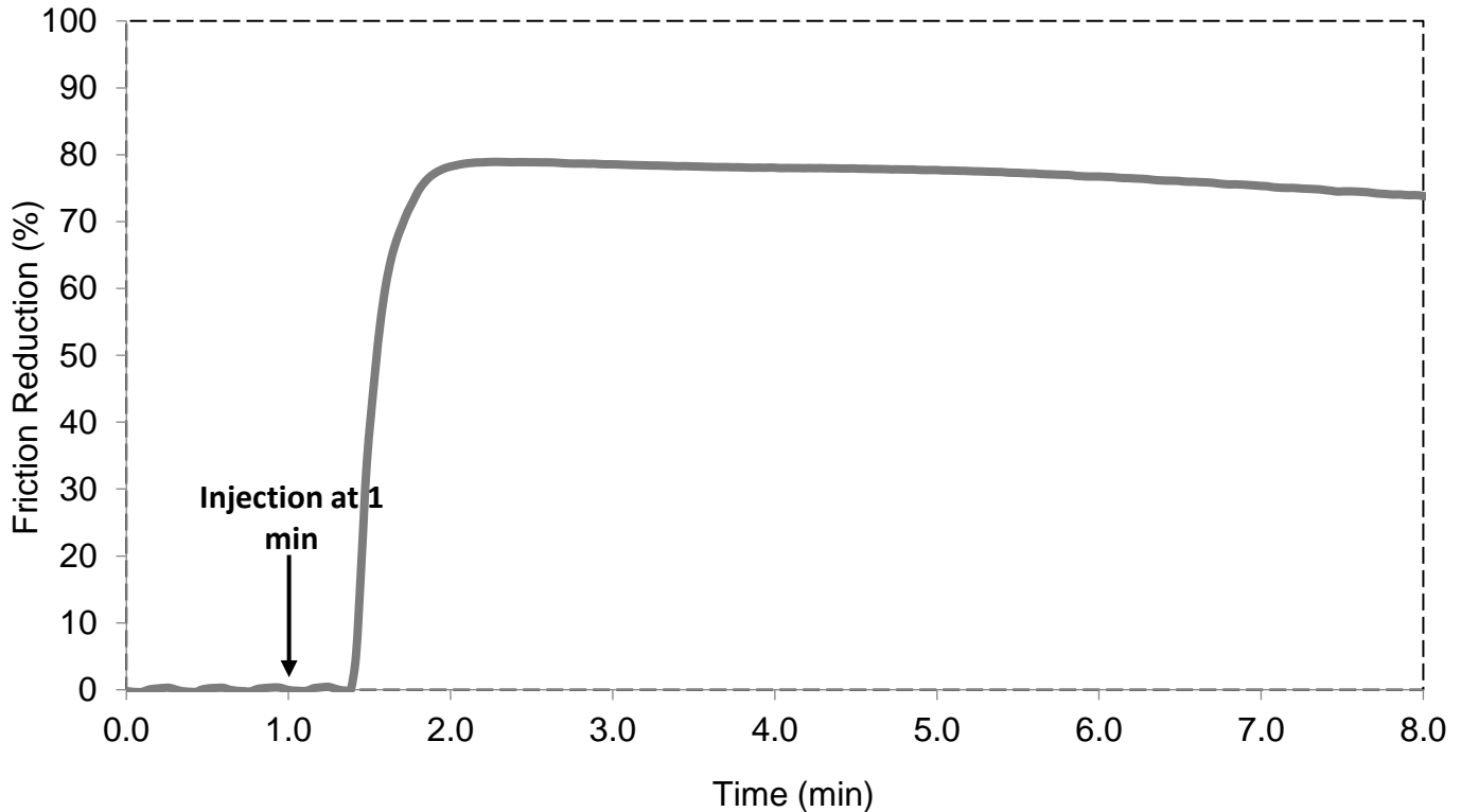
Figure 2. FR performance of TS-EH in 150K TDS Marcellus Brine.
