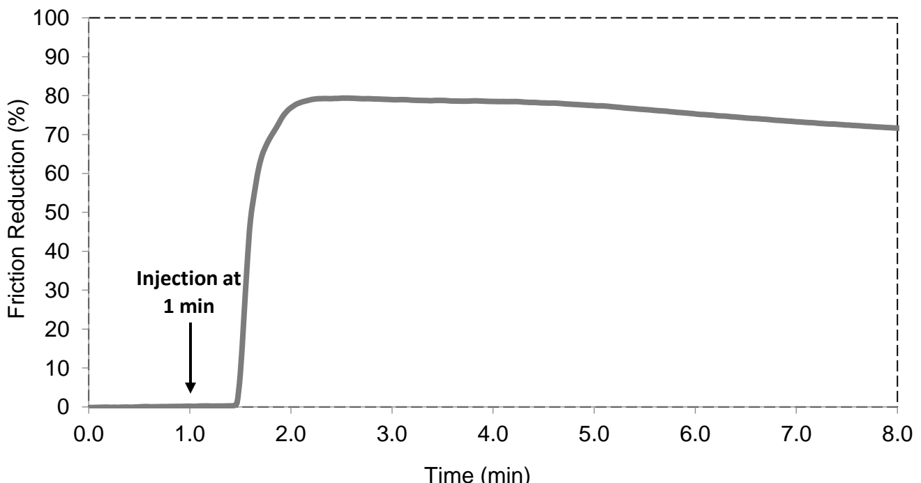
Figure 1. FR performance of TS-EH in 108K TDS API Brine
