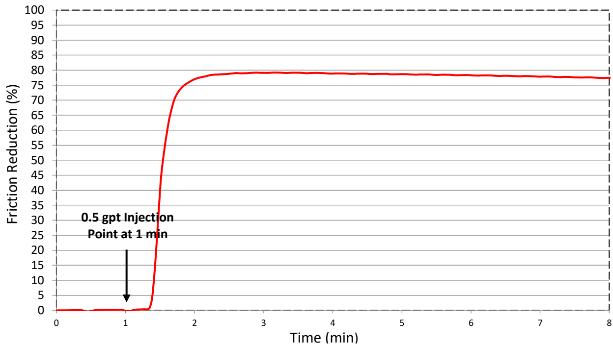
Figure 2. FR performance of TEXAN DRY-FRESH in API 108 K brine at room temperature
